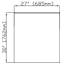
EDWR(F)27-B Front
