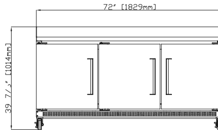
EDWR(F)72-B Front
