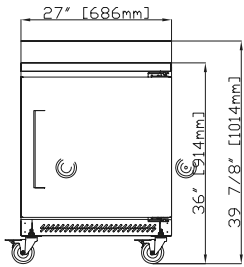
EDWR(F)27-B Front
