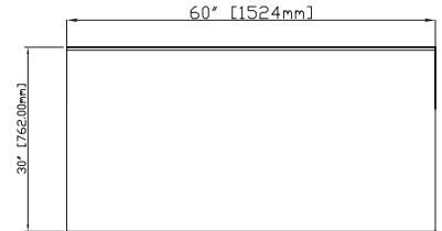
EDWR60-B Front
