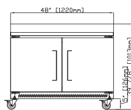
EDWR(F)48-B Front
