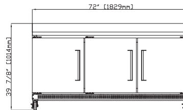
EDWR(F)-72-B Front
