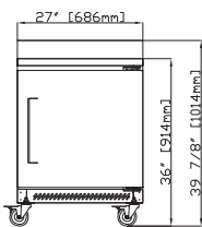
EDWR(F)27-B Front
