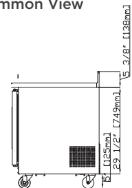
EDWR(F)-B Side Common View
