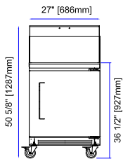
EDMT27-12 Front
