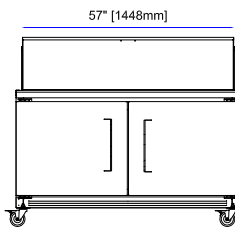
EDMT60-24 Front
