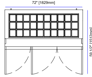
EDMT70-32 Front
