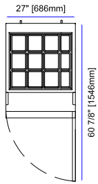
EDMT27-12 Front
