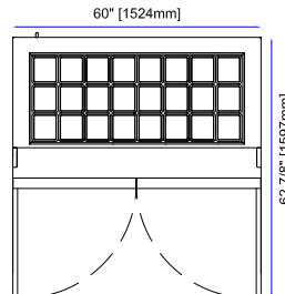
EDMT60-24 Front
