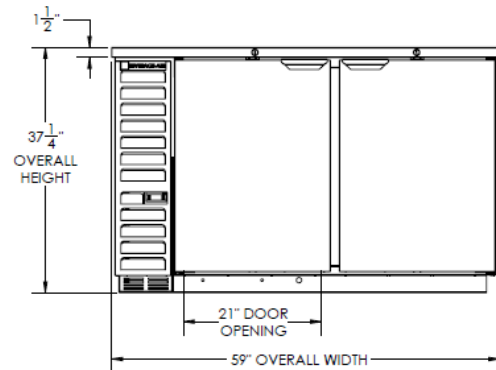
Elevation View
