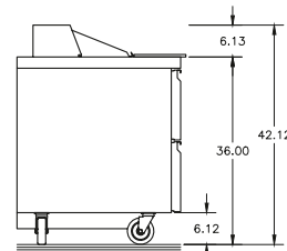
4427NP-8 Left Side View
