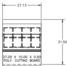
4427NP-6 Elevation View
