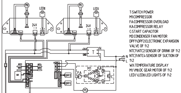
ELECTRIC WIRING DIAGRAM(MyGranita-2S)
