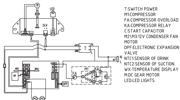
ELECTRIC WIRING DIAGRAM(MyGranita-1S)
