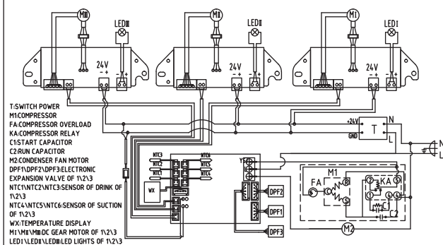
ELECTRIC WIRING DIAGRAM(MyGranita-3S)
