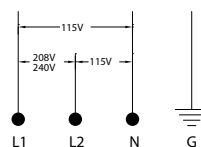
Single Phase
