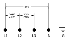
Three Phase
