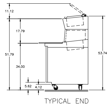
TYPICAL END
