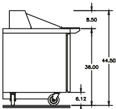
4448NP-12M Left Side View
