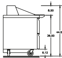
D4448NP-12M Left Side View
