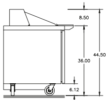
4464NP-18M Right Side View
