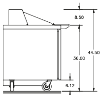
4472NP-18M Right Side View
