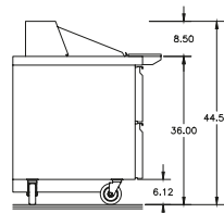
D4472NP-18M Right Side View
