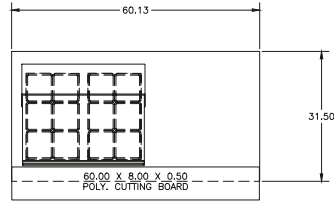
D4460NP-12M Pan Cutout Configuration
