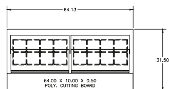
D4464NP-16 Pan Cutout Configuration
