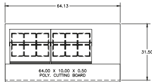
4464NP-12 Pan Cutout Configuration
