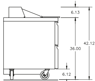
D4472NP-18 Side View
