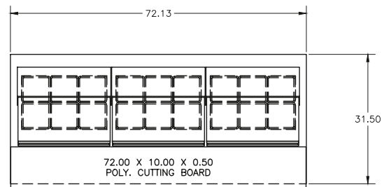
D4472NP-18 Pan Cutout Configuration
