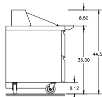
D4472NP-24M Right Side View
