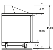
4472NP-24M Right Side View
