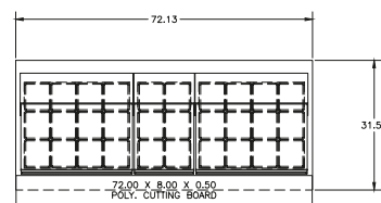
D4472NP-30M Pan Cutout Configuration
