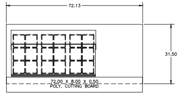
D4472NP-18M Pan Cutout Configuration
