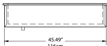
Elevation View N8046N
