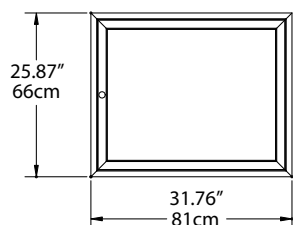
Plan View N8231G
