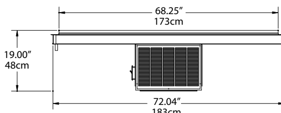
Elevation View N8273G
