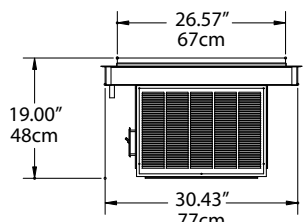
Elevation View N8231G
