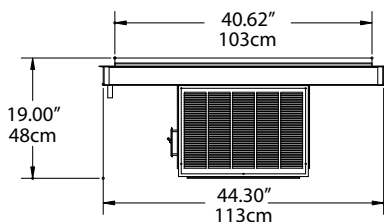
Elevation View N8245G
