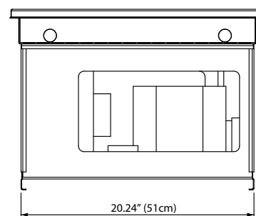
Right End View N8200-ST Models
