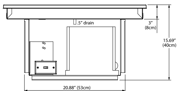
Elevation View N8200-ST Models
