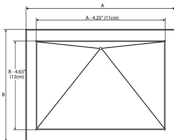
Plan View N8200-ST Models
