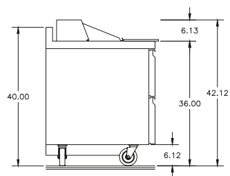
STD4460NP-8 Side View
