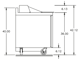
ST4460NP-8 Side View
