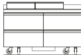
STD4464NP-12 Elevation View
