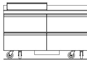
STD4464NP-8 Elevation View
