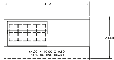
ST4464NP-8 Pan Cutout Configuration
