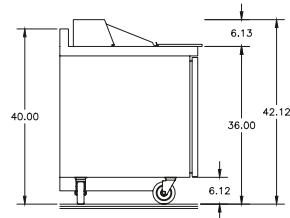
ST4464NP-12 Right Side View
