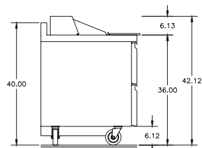
STD4464NP-8 Right Side View
