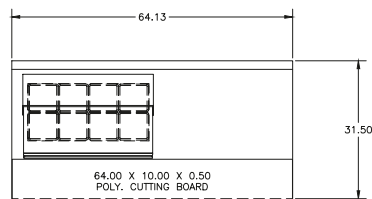
STD4464NP-8 Pan Cutout Configuration
