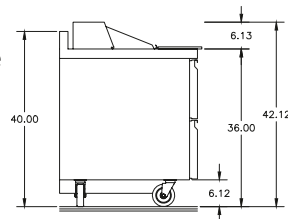
STD4464NP-12 Right Side View
