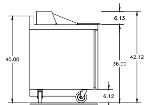
ST4464NP-8 Side View
