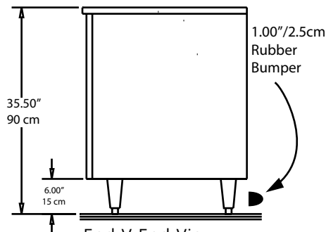
End View Models UC4048P
