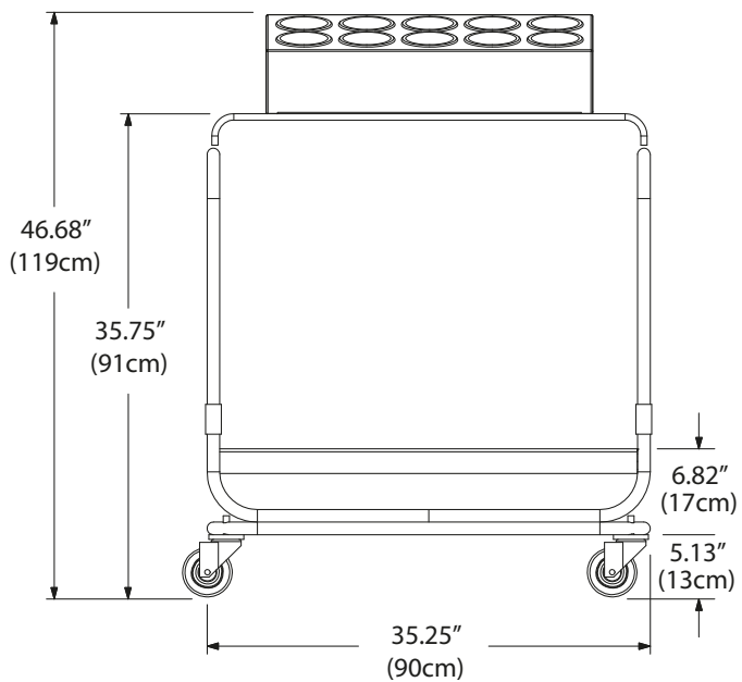
Elevation View UTS-1 & UTS-1SS
