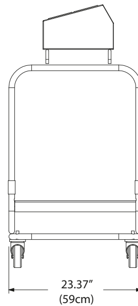
Side View UTS-1 & UTS-1SS
