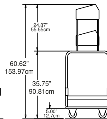
RIGHT END VIEW MODELS UTSP-2, & UTSP-2SS
