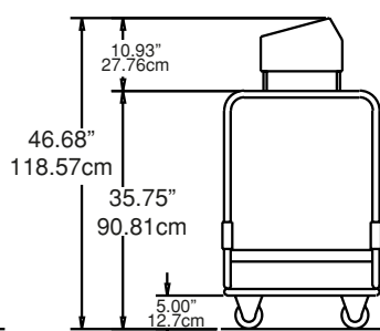
RIGHT END VIEW MODELS UTSP-1 & UTSP-1SS
