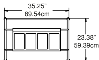
PLAN VIEW MODELS UTSP-2 & UTSP-2SS
