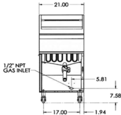
1GR65M Front
