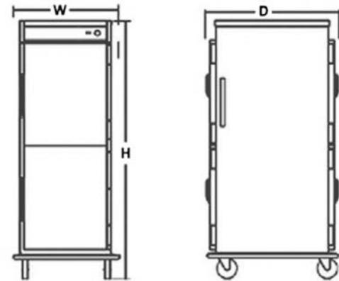
VPT15 Front & Side Views
