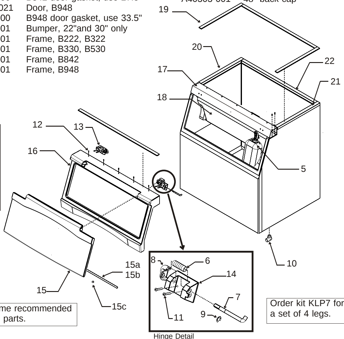
Hinge Detail
