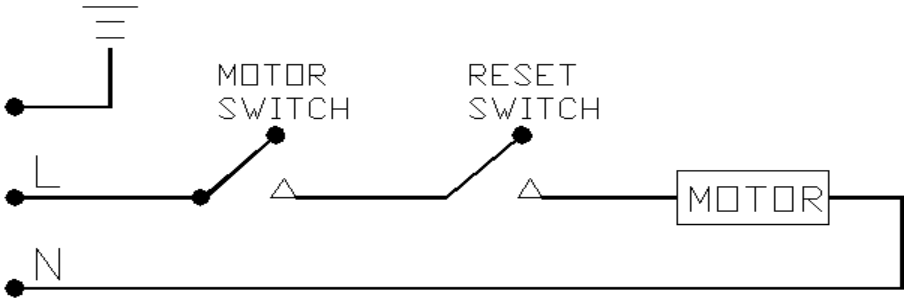
ELECTRICAL SCHEMATIC
