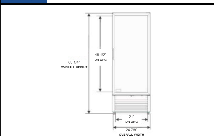
Elevation View
