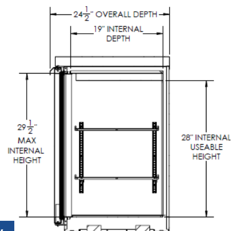
Elevation View
