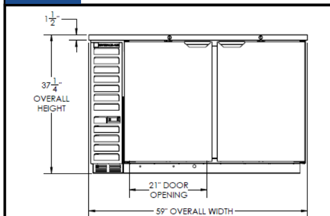
Elevation View
