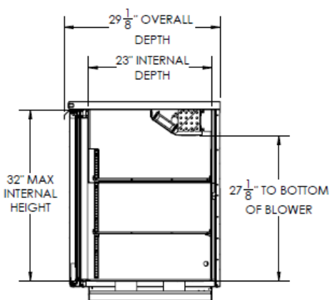
Elevation View
