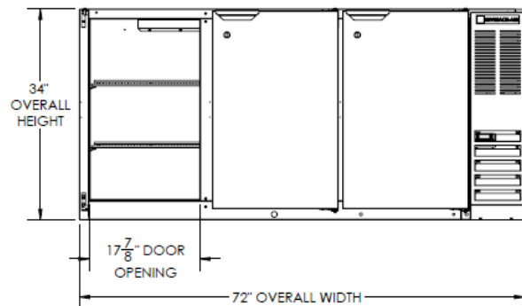
Elevation View
