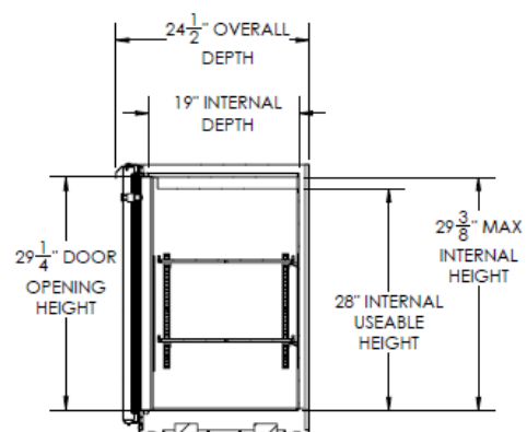
Elevation View
