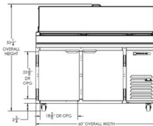
Elevation View
