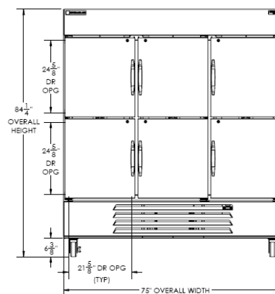
Elevation View
