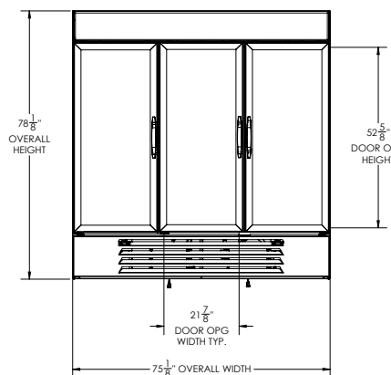
ELEVATION VIEW
