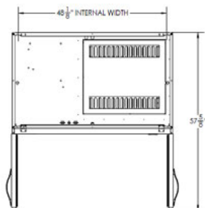
Plan View
