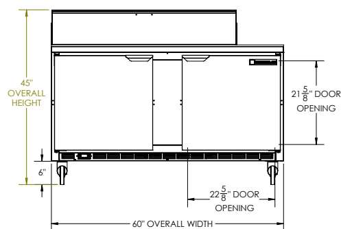
ELEVATION VIEW
