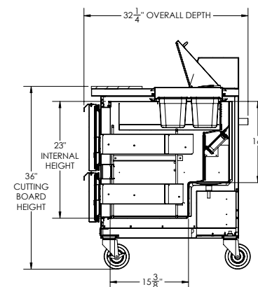
ELEVATION VIEW
