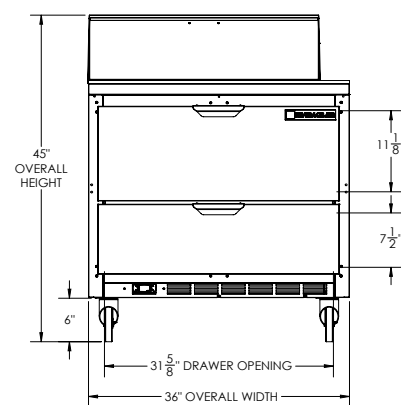
ELEVATION VIEW
