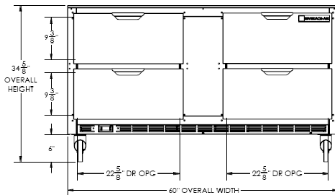
Elevation View
