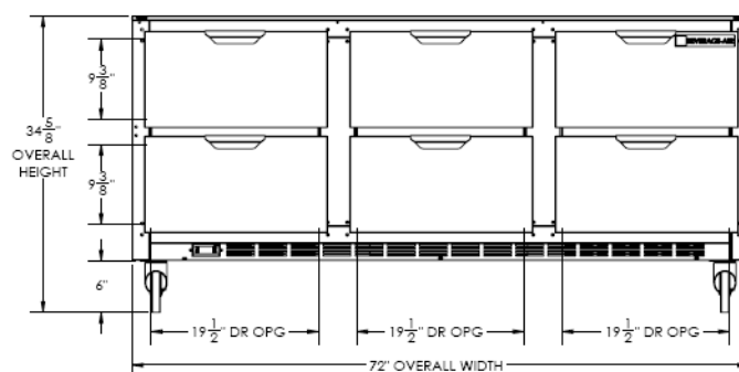
Elevation View
