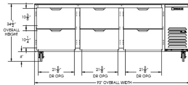
Elevation View
