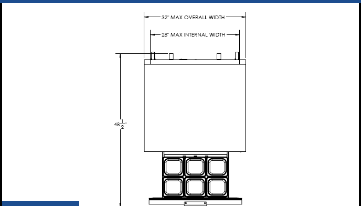
Plan View
