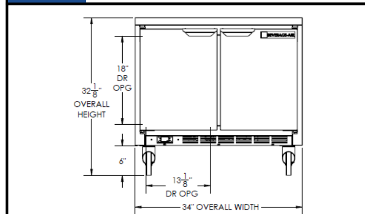
Elevation View
