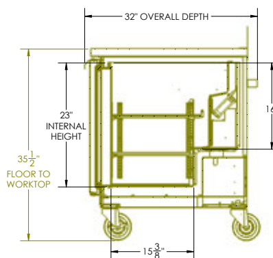
ELEVATION VIEW
