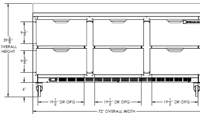
Elevation View
