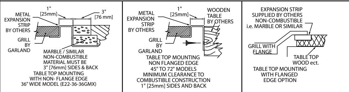
Suggested Mountings (Not to Scale)
