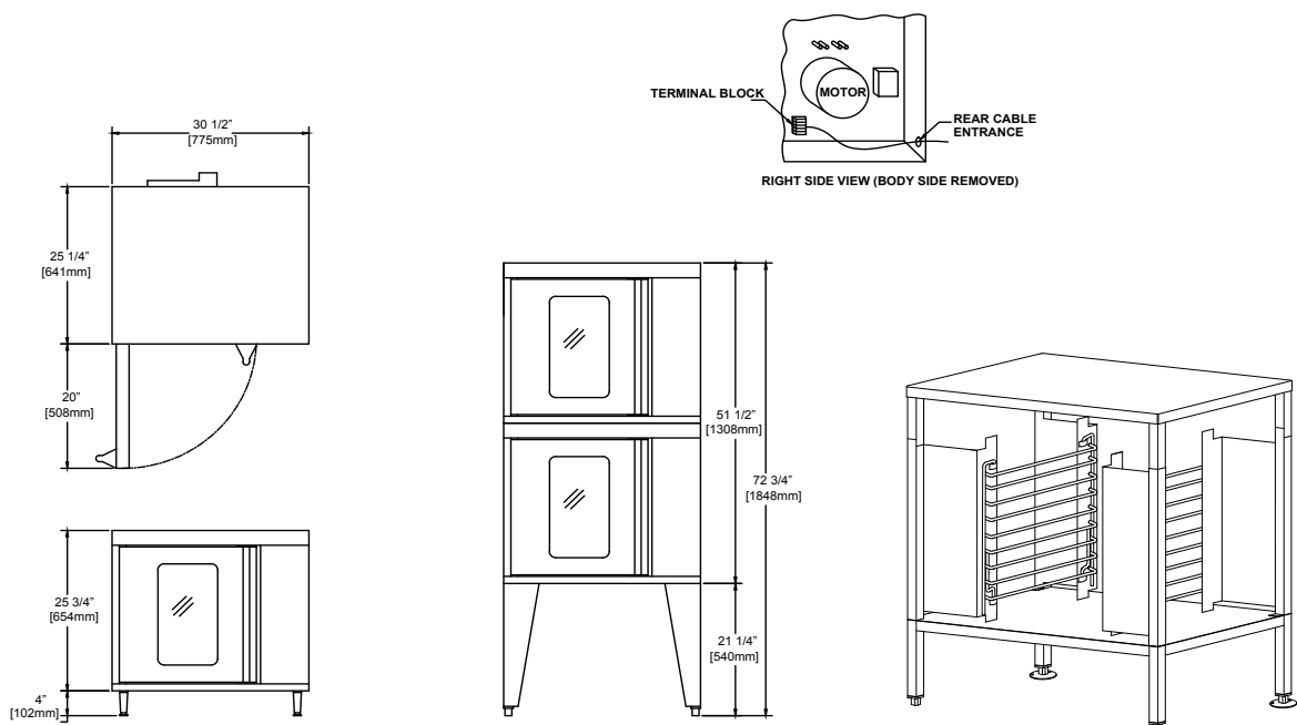
Optional equipment stand for single deck models. Stand is 34" (864mm) high.
