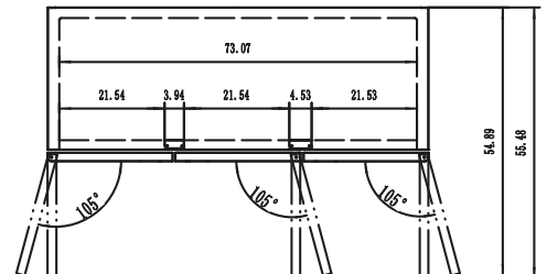
C-72RM-HC TOP VIEW
