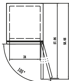
C-23RM-HC TOP VIEW
