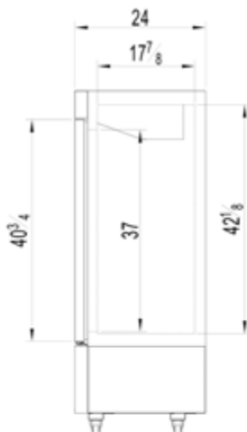
C- 10RM-HC SIDE VIEW
