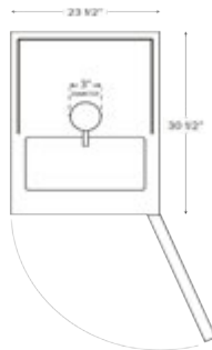
C-DD23-1-HC TOP VIEW
