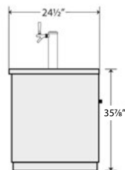
SIDE VIEW (1,2,3) DOOR MODELS
